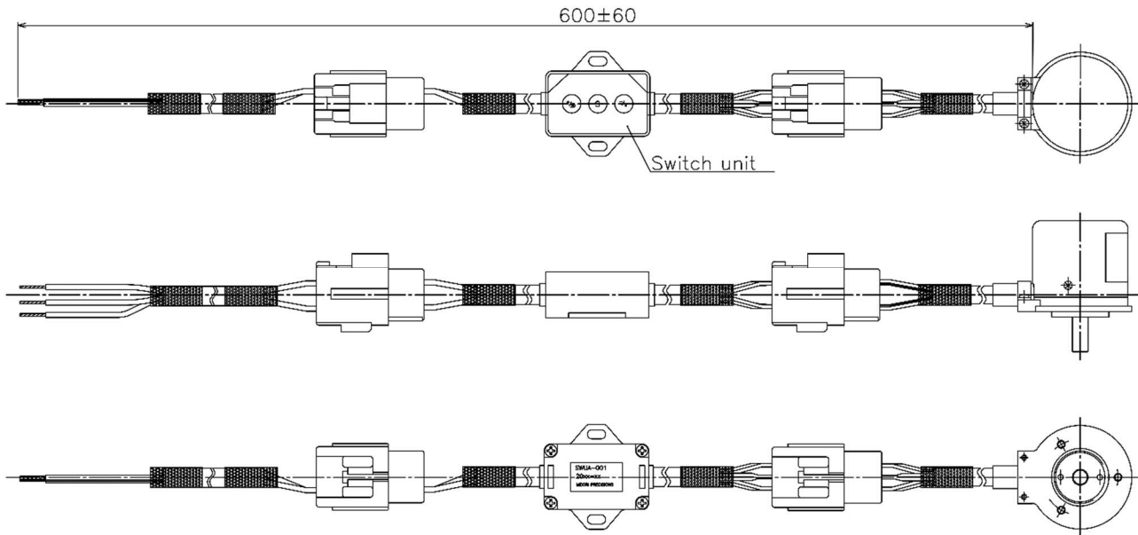
Detachable Cable type, all connected
