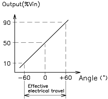
Voltage Ratio
